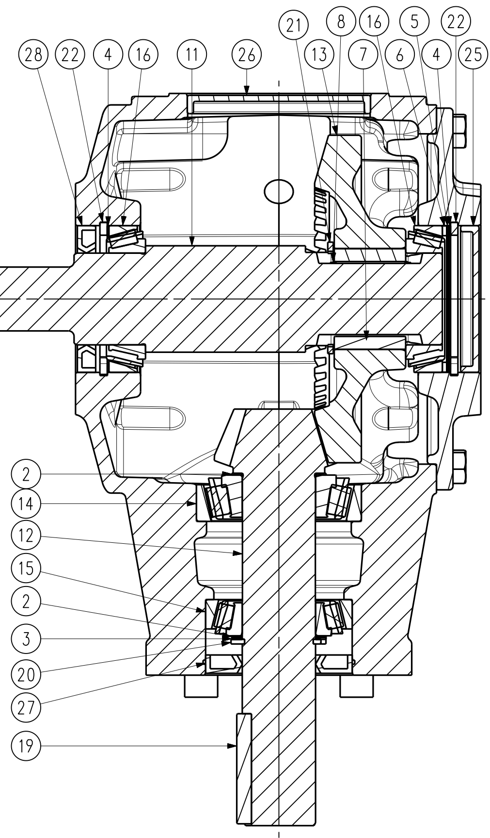
SEZ./SECT. A-A
