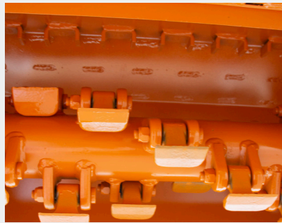
Internal counter combs
