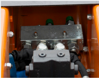
Fluid box allowing correct flow to motor
