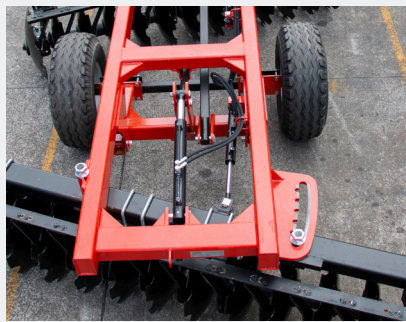
Hydraulic angle adjustment on rear gang
